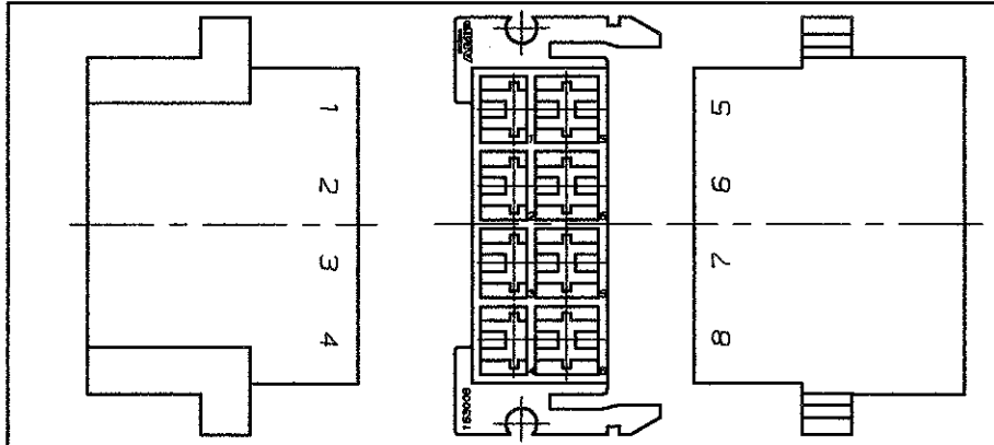
THESE VIEWS SHOW THE EXTRA NUMBERING FOR: 1-163008-0
