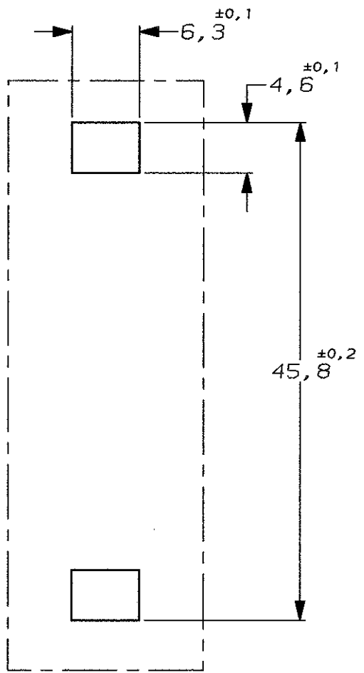
PANEL (1,4 MAX. TH.) CUT-OUT
